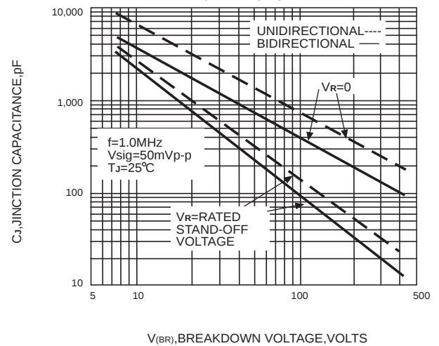
FIG. 4-TYPICAL JUNCTIONAL CAPACITANCE UNIDIRECTIONAL
